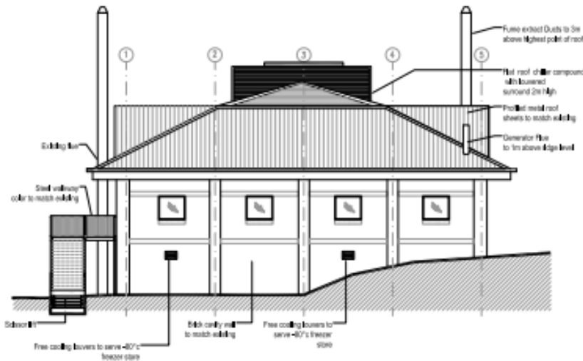
Proposed East Elevation 1:200 @A3
