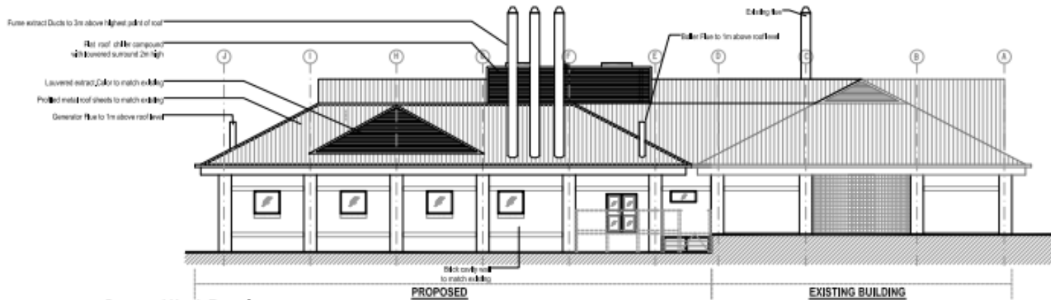
Proposed North Elevation 1:200 @A3
